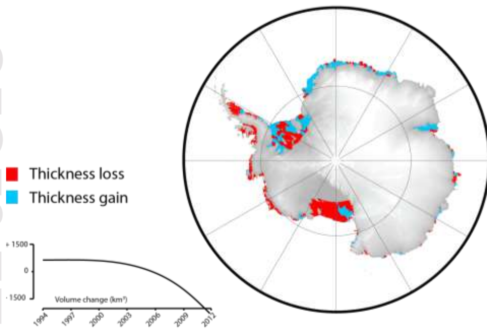
Figure 2. Observed thickness change of all ice-shelves around the Antarctic continent with colours showing the absolute change per decade between 1994 and 2012. Modified from Paolo et al., 2015 37 and 2016 38 .
