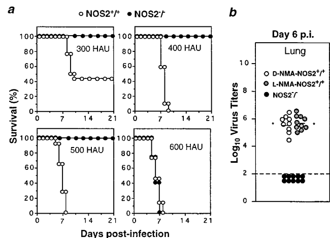
Figure 1. Disruption of NOS2 confers a protective effect during influenza A virus infection. (a) Mortality in male NOS2^{+/+} or NOS2^{-/-} mice ( n = 20 per group at each dose) inoculated intranasally with 300, 400, 500, or 600 HAU influenza A (strain A/PR/8/34) and monitored for 21 d. Data represent four independent experiments. (b) Lung influenza A titers in d-NMA- or 1-NMA-treated NOS2^{+/+} mice and NOS2^{-/-} mice intranasally infected with 400 HAU of virus and determined at day 6 after infection. Dashed line, Assay detection limit. Data are derived from three experiments and expressed as log 10 virus titers/gram tissue \pm SEM. * P < 0.01 versus NOS2^{-/-} group, unpaired t test.
