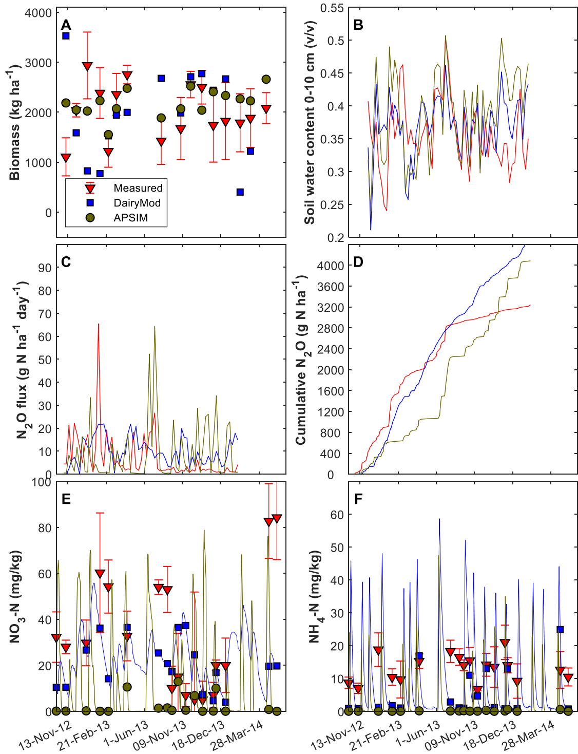
Fig. 1. Simulated and measured (A) pasture biomass, (B) weekly average soil water content, (C) cumulative weekly N 2 O flux rate, (D) cumulative daily N 2 O emissions, (E) soil NO 3 and (F) soil NH 4 from 14 October 2012 to 13 May 2014 at Camden, NSW, Australia.
