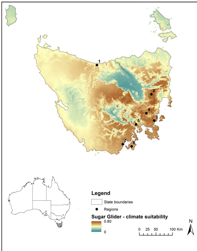
Figure 1 MAXENT model of bioclimatic suitability for sugar gliders across the study area, showing the location of the seven regions where swift parrot nests were monitored. The swift parrot nesting regions (and the number of nests included in the nest survival analysis from each) were as follows: (1) Devonport ( n = 7 ), (2) Eastern Tiers ( n = 15 ), (3) Wielangta ( n = 8 ), (4) Buckland ( n = 3 ), (5) Meehan Range ( n = 8 ), (6) Bruny Island ( n = 16 ) and (7) the southern forests ( n = 6 ). Note the high suitability of islands offshore the east coast of Tasmania for sugar gliders (including Region 6). Offshore islands are important breeding habitat for swift parrots, and sugar gliders are absent from these areas.
