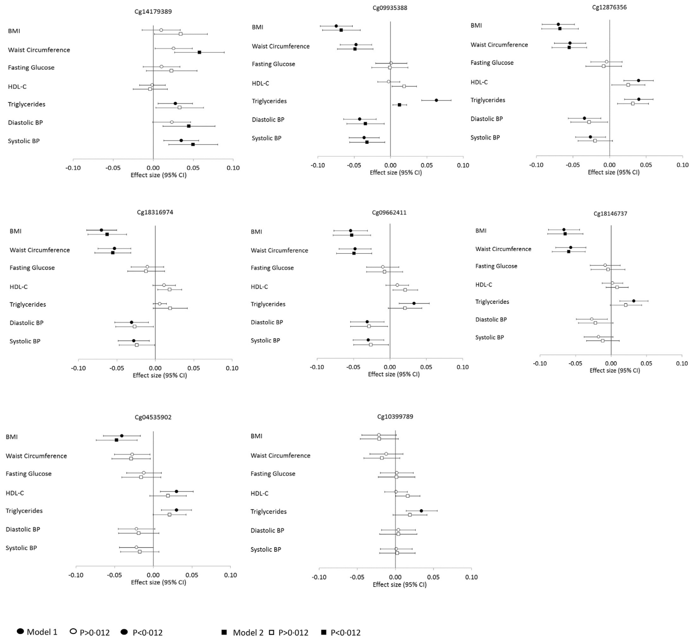
Fig. 4. Forest plot showing meta-analysis effect sizes of cardio-metabolic phenotypes in SD change by one SD lower DNA methylation at eight GFI -CpGs across all the participating studies ( n = 18,212 ). Model 1: Cardio-metabolic Phenotype = CpG + technical covariates; Model 2: Cardio-metabolic Phenotype = CpG + technical covariates + sex + adult smoking + age. Bonferroni corrected P-value threshold of P < 0.012 has been used for this analysis. Open and closed symbol indicate p > 0.012 and p < 0.012 , respectively. Standardized values with mean = 0 and standard deviation = 1 were used for cardio-metabolic phenotypes and CpG methylation across all the studies. \beta can be interpreted as SD change in cardio-metabolic phenotype per 1-SD decrease in methylation. According to availability in the participating studies, we had BMI for 18212, WC for 14665, HDL-C for 18212, TG for 18212, FG for 16529, DBP for 16529, and SBP for 16529 of the total 18212 individuals. Abbreviations: BMI – Body Mass Index, BP – Blood Pressure, CI – Confidence Interval, HDL-C – High Density Lipoprotein Cholesterol. Measurement units for each cardio-metabolic phenotype are given in Table 1.
