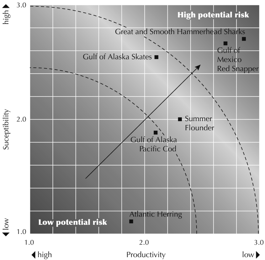
Figure 1. Productivity and susceptibility scores for selected US fisheries (Rosenberg et al. 2007). Risk increases from lower left to upper right.
