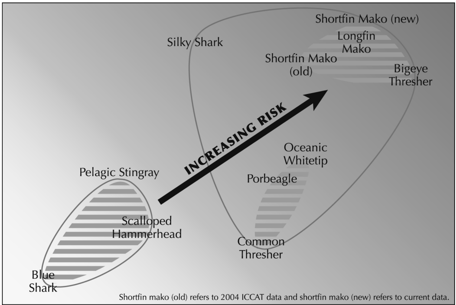
Figure 2. Results of an integrated risk assessment for Atlantic shark and ray species taken in pelagic fisheries (Simpfendorfer et al. 2008). Risk increases from lower left to upper right, and represents the risk of overexploitation by pelagic longline fisheries in the Atlantic Ocean. The axes are dimensionless, because the results are derived from multi-dimensional scaling.
