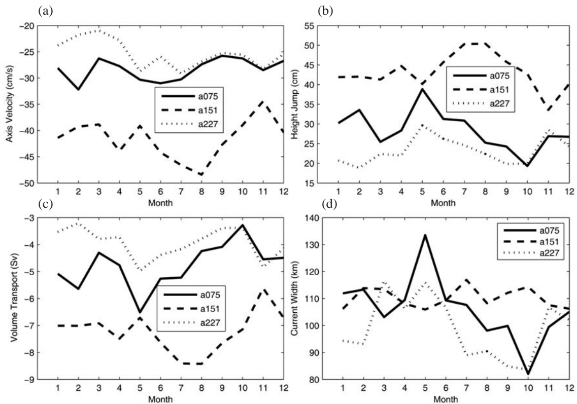
Fig. 8. Monthly averaged axis velocity (a), height jump (b), geostrophic volume transport (c), and width (d) of the LC from January 1993 to August 2002 for three tracks a075, a151, and a227. Negative velocities (a) indicate that they are left of the track, when looking along the track from north to south. Negative transports (c) mean the current is southward and 1 \text{ Sv} = 10^6 \text{ m}^3 \text{ s}^{-1} .
