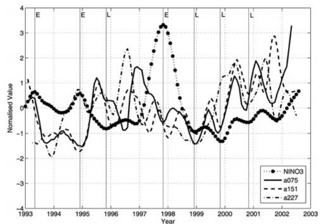
Fig. 11. Normalised time-series of NINO3 SST anomalies and geostrophic volume transports for tracks a075, a151, and a227. Vertical solid lines indicate the year of ENSO events, from which "E" and "L" mark the peaks of El Niño and La Niña years, respectively.
