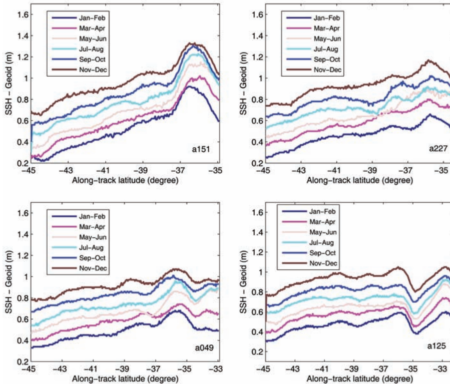
Fig. 4. Bimonthly averaged along-track ocean dynamic heights along four ascending tracks a151, a227, a049, and a125. Stacked plots are offset by 0.1 m with Jan-Feb values (the lowest curve) being true.
