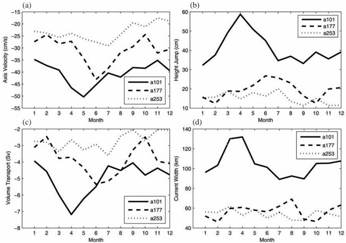
Fig. 7. Monthly averaged axis velocity (a), height jump (b), geostrophic volume transport (c), and width (d) of the LC from January 1993 to August 2002 for three tracks a101, a177, and a253. Negative velocities (a) indicate that they are left of the track, when looking along the track from north to south. Negative transports (c) mean the current is southward and 1 \text{ Sv} = 10^6 \text{ m}^3 \text{ s}^{-1} .
