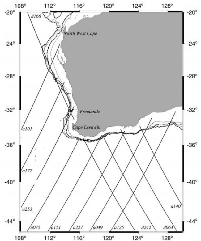
Fig. 2. Distribution of selected T/P tracks over the western and southern Australian coastal regions. The contours show the bathymetric depth from 500 m to 2000 m along the continental shelf edge. The affixes "a" and "d" before the track numbers denote an ascending and descending track, respectively. The satellite orbits from south to north along the ascending track and vice versa along the descending track.
