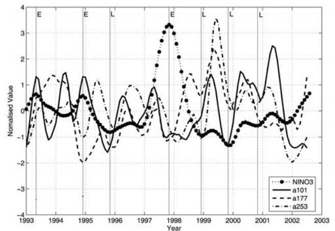
Fig. 10. Normalised time-series of NINO3 SST anomalies and geostrophic volume transports for tracks a101, a177, and a253. Vertical solid lines indicate the year of ENSO events, from which "E" and "L" mark the peaks of El Niño and La Niña years, respectively.
