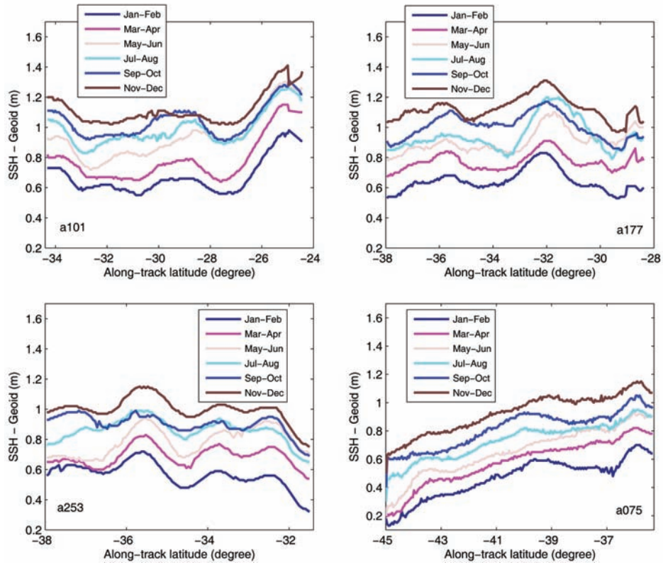
Fig. 3. Bimonthly averaged along-track ocean dynamic heights along four ascending tracks a101, a177, a253, and a075. Stacked plots are offset by 0.1 m with Jan-Feb values (the lowest curve) being true.
