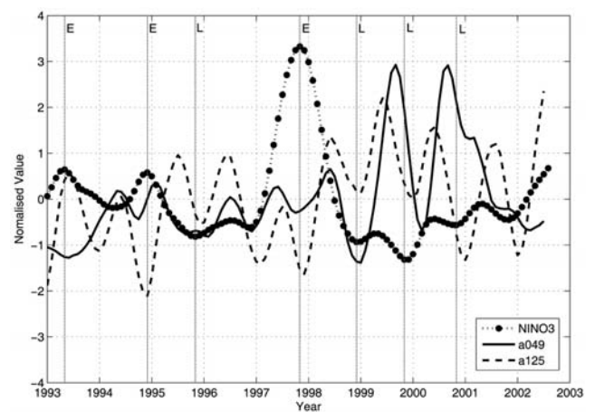
Fig. 12. Normalised time-series of NINO3 SST anomalies and geostrophic volume transports for tracks a049, and a125. Vertical solid lines indicate the year of ENSO events, from which "E" and "L" mark the peaks of El Niño and La Niña years, respectively.
