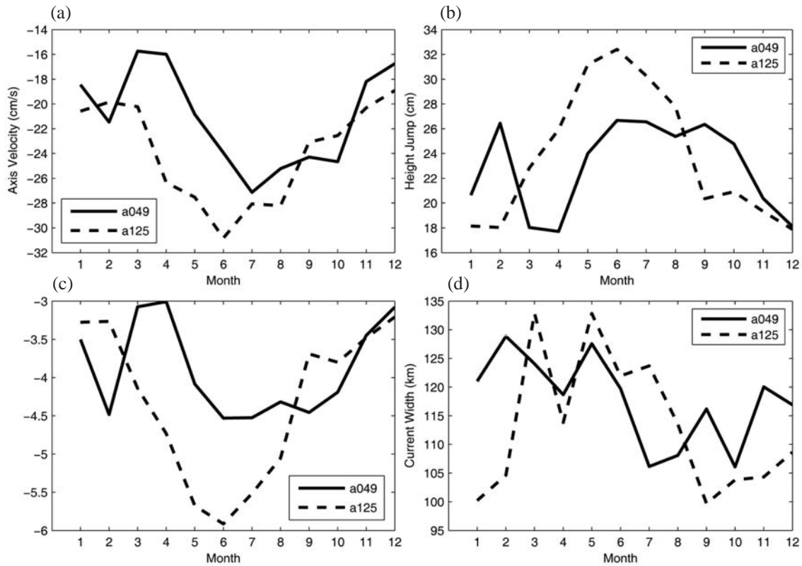
Fig. 9. Monthly averaged axis velocity (a), height jump (b), geostrophic volume transport (c), and width (d) of the LC from January 1993 to August 2002 for three tracks a049, and a125. Negative velocities (a) indicate that they are left of the track, when looking along the track from north to south. Negative transports (c) mean the current is southward and 1 \text{ Sv} = 10^6 \text{ m}^3 \text{ s}^{-1} .
