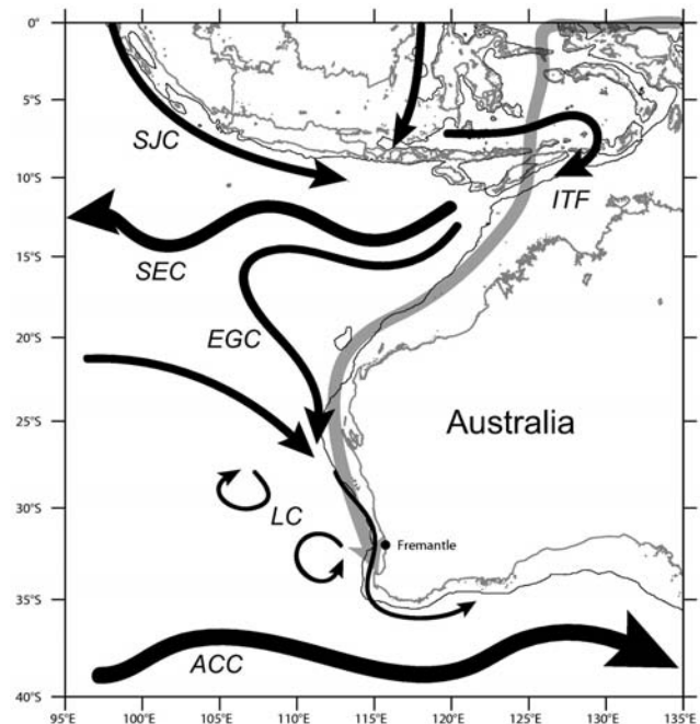
Fig. 1. Schematic of the major surface currents in the east-southeast Indian Ocean (adapted from Feng et al. 2003). ITF: Indonesian Through-flow; SEC: South Equatorial Current; SJC: South Java Current; EGC: East Gyral Current; LC: Leeuwin Current; ACC: Antarctic Circumpolar Current. The meandering of the SEC and the Leeuwin Current eddies are also sketched. A shaded, transparent arrow is used to highlight the waveguide along which the Pacific ENSO signals propagate.
