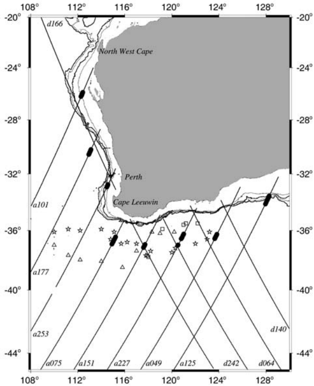
Fig. 6. Monthly averaged axis locations (highlighted by solid circles) of the LC at each T/P track in the region west and south of WA from January 1993 to August 2002. Symbols of triangle, star and square are approximately monthly positions of migrating (from east to west) eddies A, B, and C, respectively, from Cresswell and Griffin (2004, Fig. 13).
