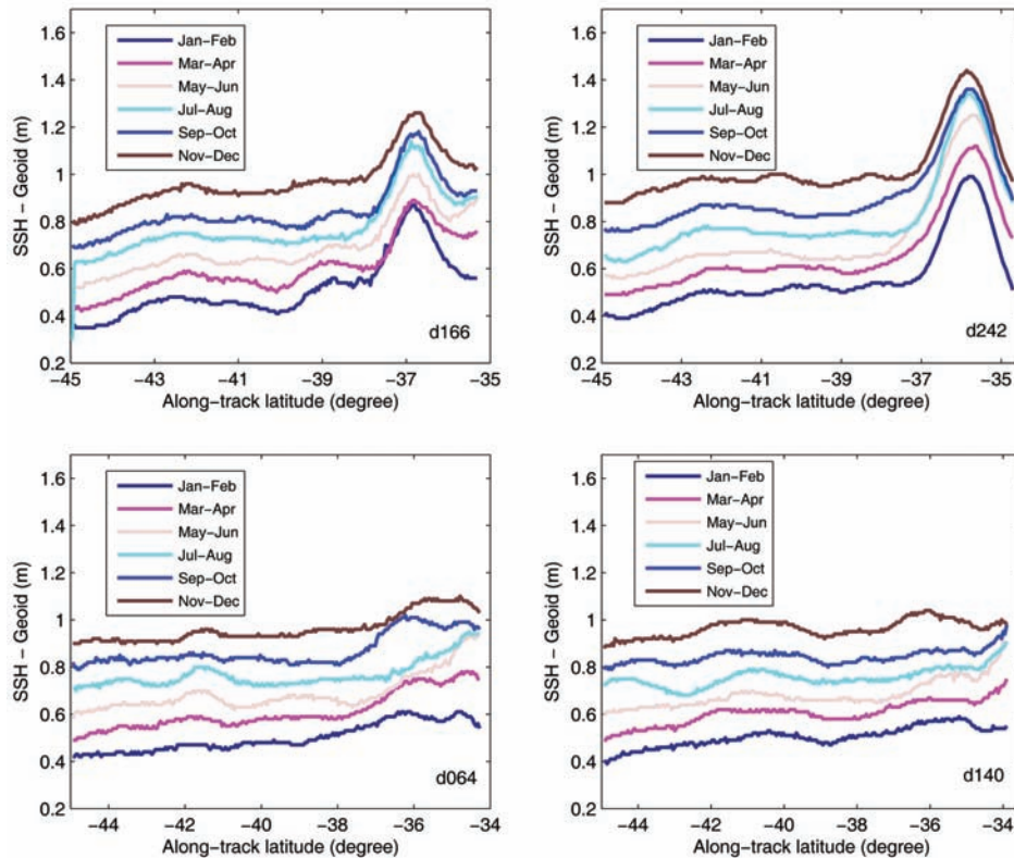
Fig. 5. Bimonthly averaged along-track ocean dynamic heights along four descending tracks d166, d242, d064, and d140. Stacked plots are offset by 0.1 m with Jan-Feb values (the lowest curve) being true.
