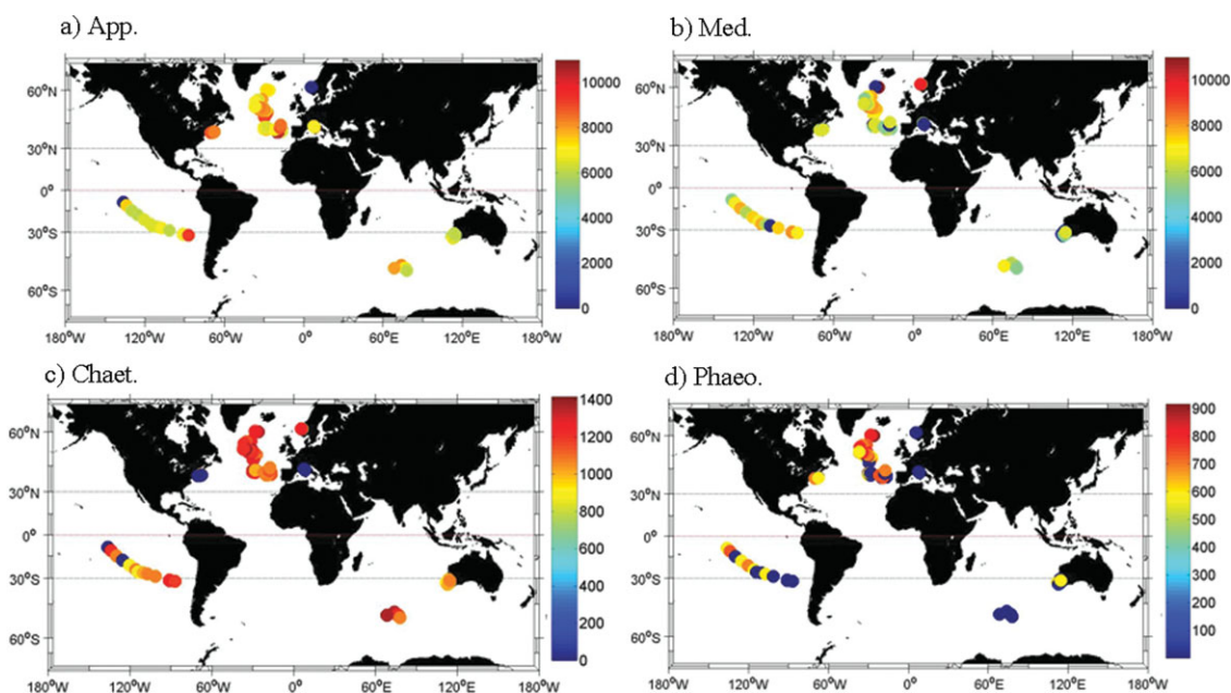
Figure 7. Maps of abundance ( \text{ind. } \text{m}^{-2} ) of selected macrozooplankton groups.
