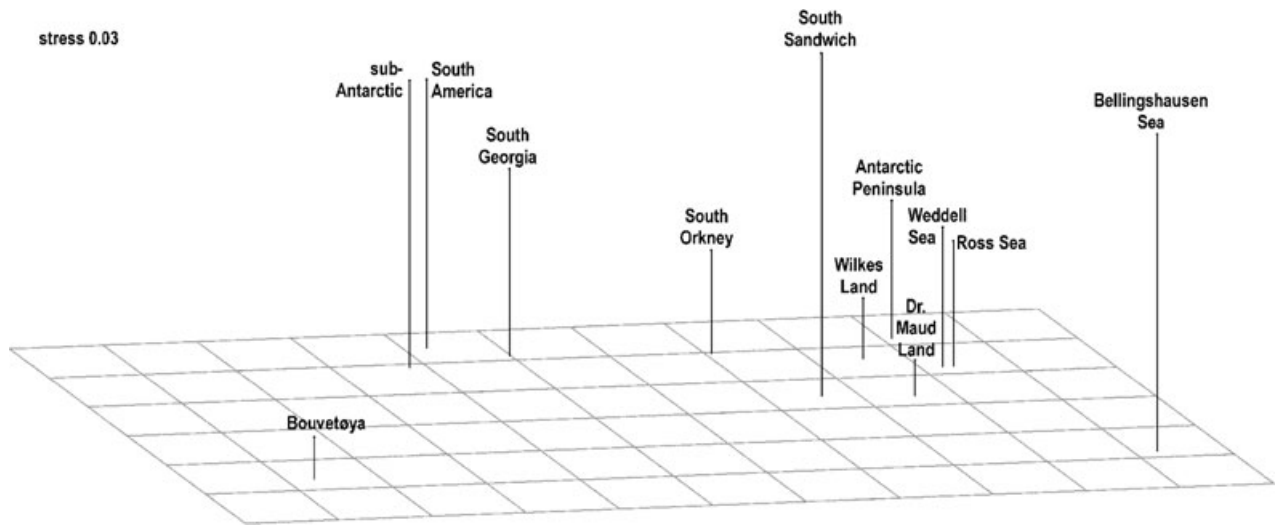
Fig. 3 Multi-dimensional scaling ordination analysis of Antarctic sectors, the sub-Antarctic region and the South America region.
