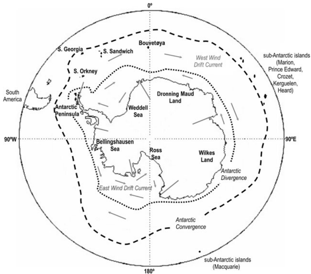
Fig. 1 Outlines of the Antarctic. The sectors considered in this work are marked in boldface.
