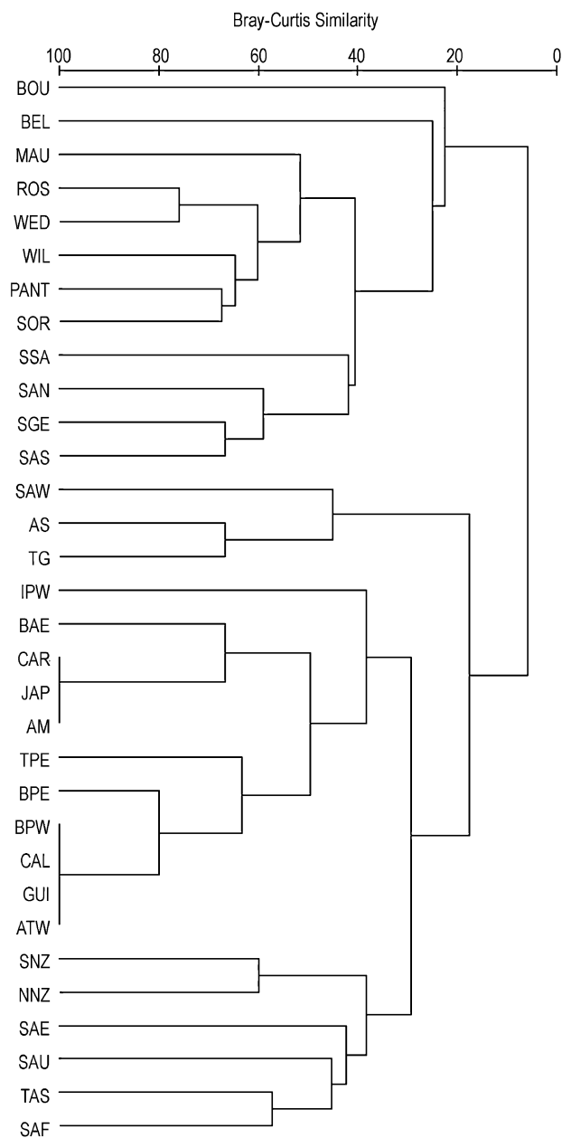
Fig. 2 Bray-Curtis classification analysis. Abbreviations: BOU, Bouvetøya; BEL, Bellingshausen Sea; MAU, Dronning Maud Land; ROS, Ross Sea; WED, Weddell Sea; WIL, Wilkes Land; PANT, Antarctic Peninsula; SOR, South Orkney Islands; SSA, South Sandwich Islands; SAN, sub-Antarctic region; SGE, South Georgia Islands; SAS, South America Region; SAW, western South America Region; AS, Amsterdam–Saint Paul; TG, Tristan da Cunha; IPW, Indo-West Pacific region; BAE, eastern Atlantic Boreal region; CAR, Carolina region; JAP, Japan region; AM, Mediterranean–Atlantic region; TPE, eastern Pacific region; BPE, eastern Pacific Boreal region; BPW, western Pacific Boreal region; CAL, California region; GUI, eastern Atlantic region; ATW, western Atlantic region; SNZ, southern New Zealand region; NNZ, northern New Zealand region; SAE, eastern South America region; SAU, southern Australia region; TAS, Tasmania region; SAF, southern Africa region.
