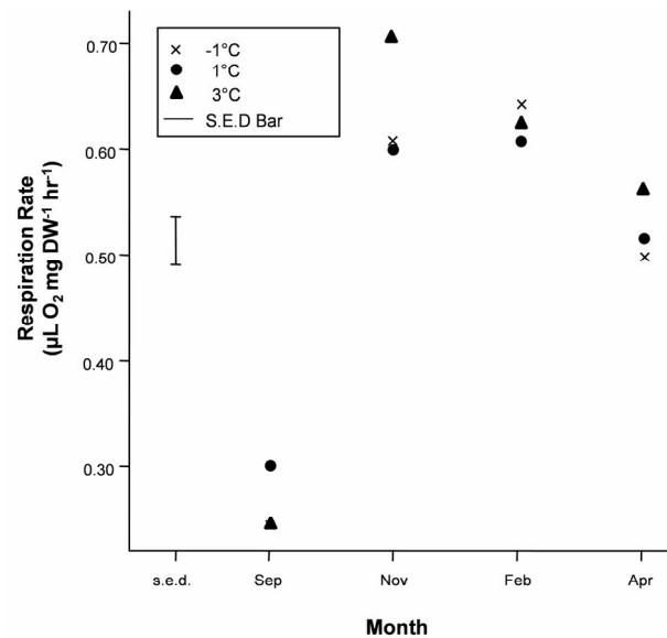
Figure 3. Mean respiration rates on a dry weight (DW) basis ( \mu\text{L O}_2 \text{ mg}\cdot\text{DW}^{-1}\cdot\text{hr}^{-1} ) for the temperature treatment ( -1^\circ\text{C} , 1^\circ\text{C} and 3^\circ\text{C} ). The Standard Error of Difference bar (s.e.d) is based on the residual mean square (m.s.) given in Table 2 and the sample of four krill in each treatment by month combination and gives the standard error of the pairwise differences in means for a given month. Any differences that are more than twice the length of the s.e.d. bar based on a t-statistic of 2.0 can be considered significant at the 95% level.
