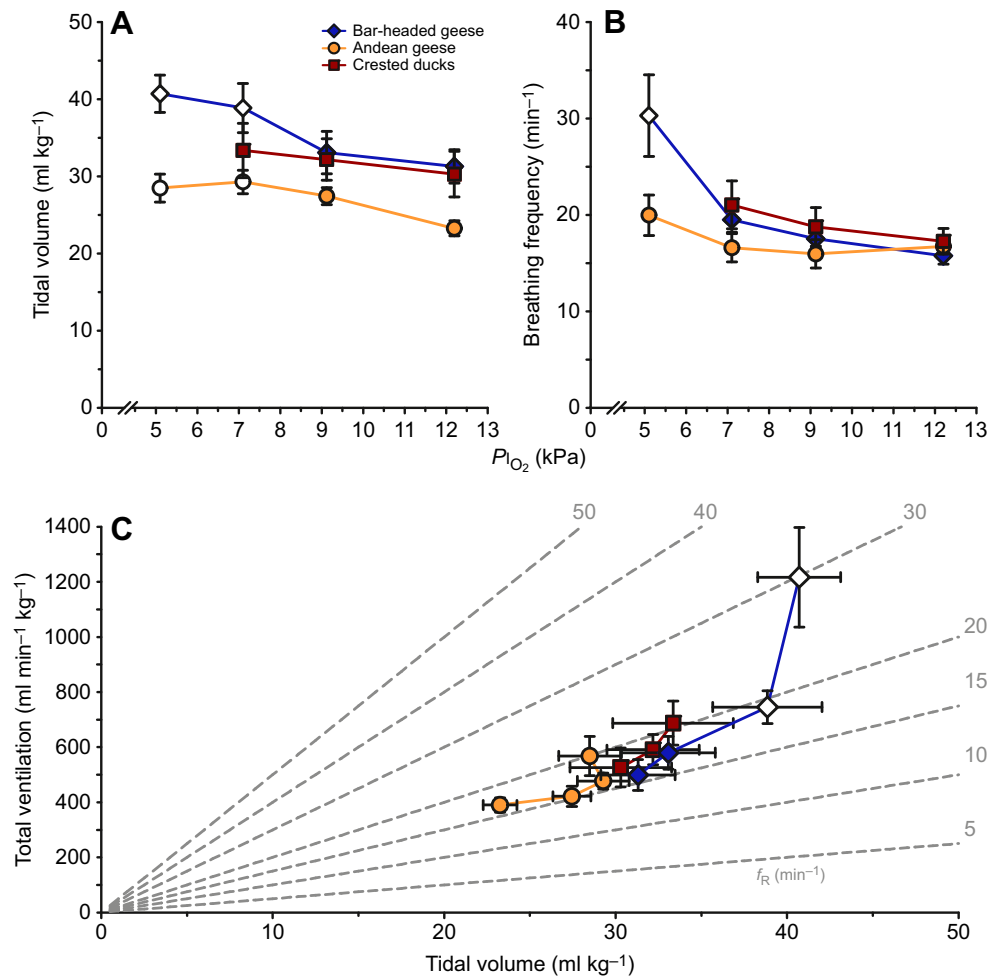
Fig. 2. Hypoxic ventilatory response patterns. (A,B) The relationship between inspired partial pressure of oxygen ( P_{I_{O_2}} ) and (A) tidal volume (in BTPS) and (B) breathing frequency. (C) Changes in total ventilation (in BTPS) and its components, tidal volume (x-axis) and breathing frequency ( f_R ; dashed isopleths), during exposure to progressive hypoxia. All values represent means \pm s.e.m. (bar-headed geese, N=7 ; Andean geese, N=7 ; crested ducks, N=6 ). Significant differences ( P<0.05 ) in total ventilation from starting values within a species are indicated by open symbols.
