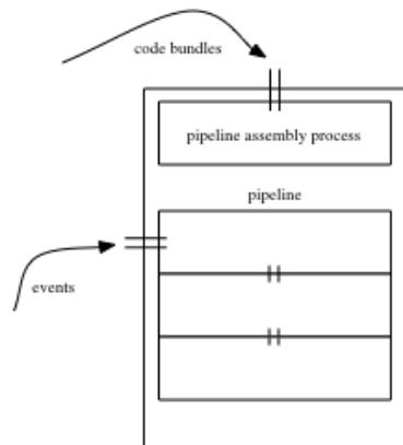
Figure 3: Pipeline deployment infrastructure.
