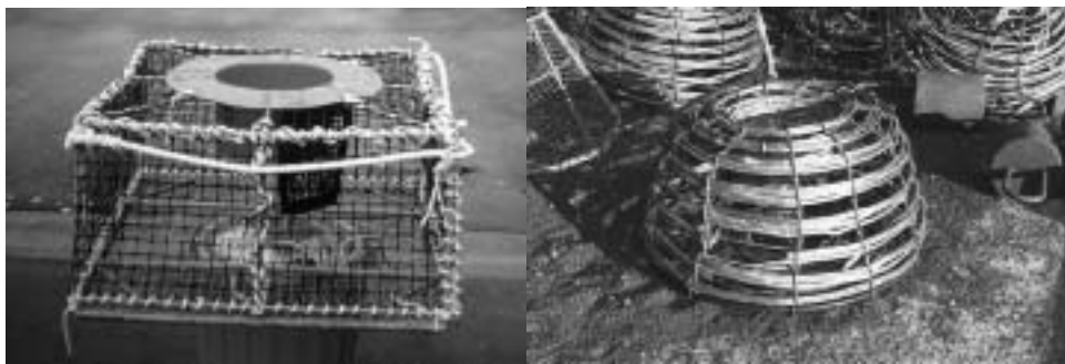
Figure 41. Steel research trap (left) and standard “beehive” trap (right) used in the commercial and recreational fisheries. Note that some fishers also use steel traps although designs differ from the research trap shown here.
