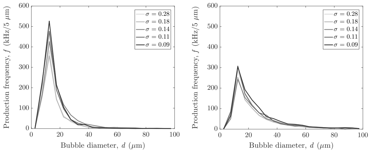
Figure 4: Production frequency histograms of the mini-tube microbubble generators across the range of tested cavitation numbers for an expansion tube length of 200 mm (left), and 100 mm (right).
